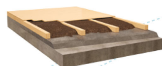
BETWEEN JOISTS LOOSE FILL
